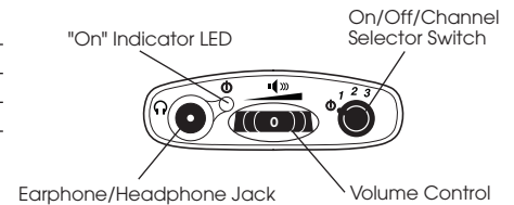
R863 Top
